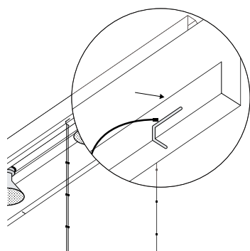
4. Cable insertion detail.
