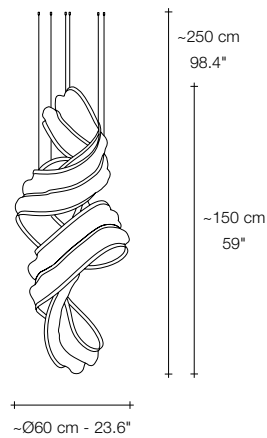
B60S On site adjustable sculpture height from 140 to 180 cm - 55.1" to 70.9" On site adjustable overall height from 240 to 300 cm - 94.5" to 118.1"
