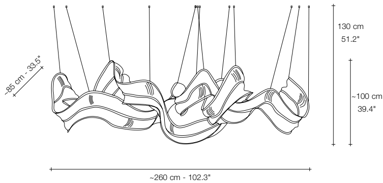
B56S On site adjustable overall height from 100 to 140 cm - 39.4" to 55.1" On site adjustable overall length from 240 to 300 cm - 94.5" to 118.1"
